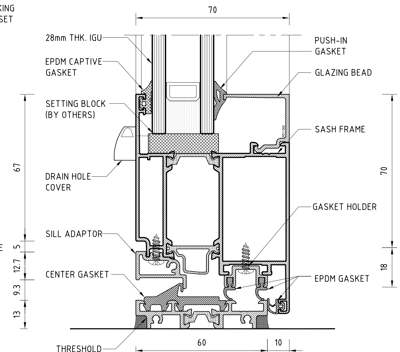
SILL DETAIL
