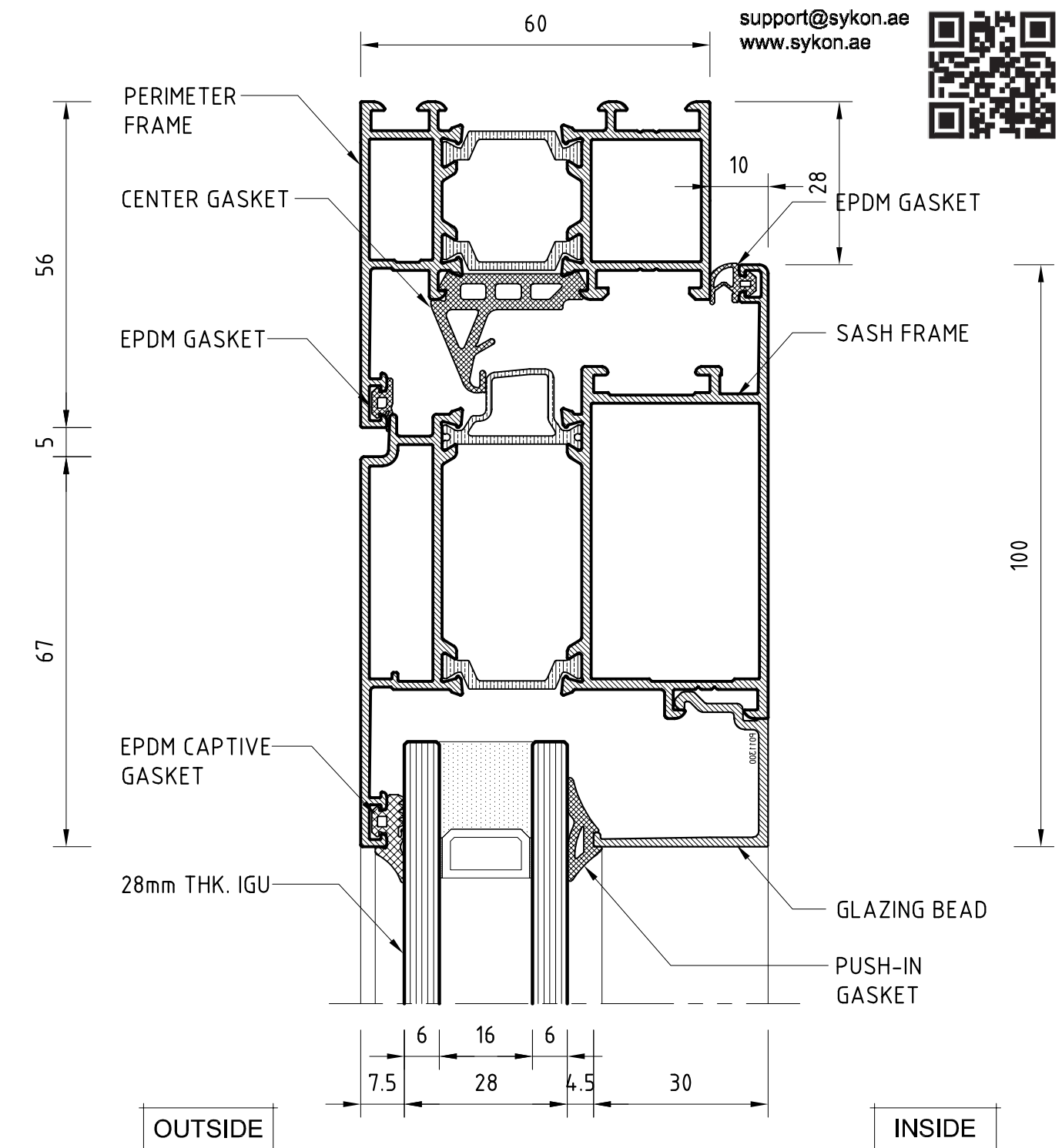
HEAD DETAIL
